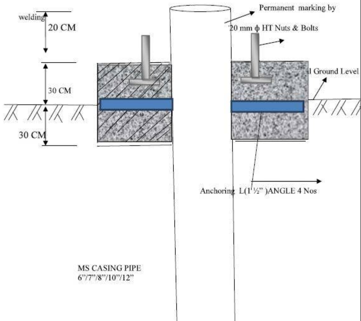
Drawing 6: A Schematic Drawing of Cement Concrete Plat Form
