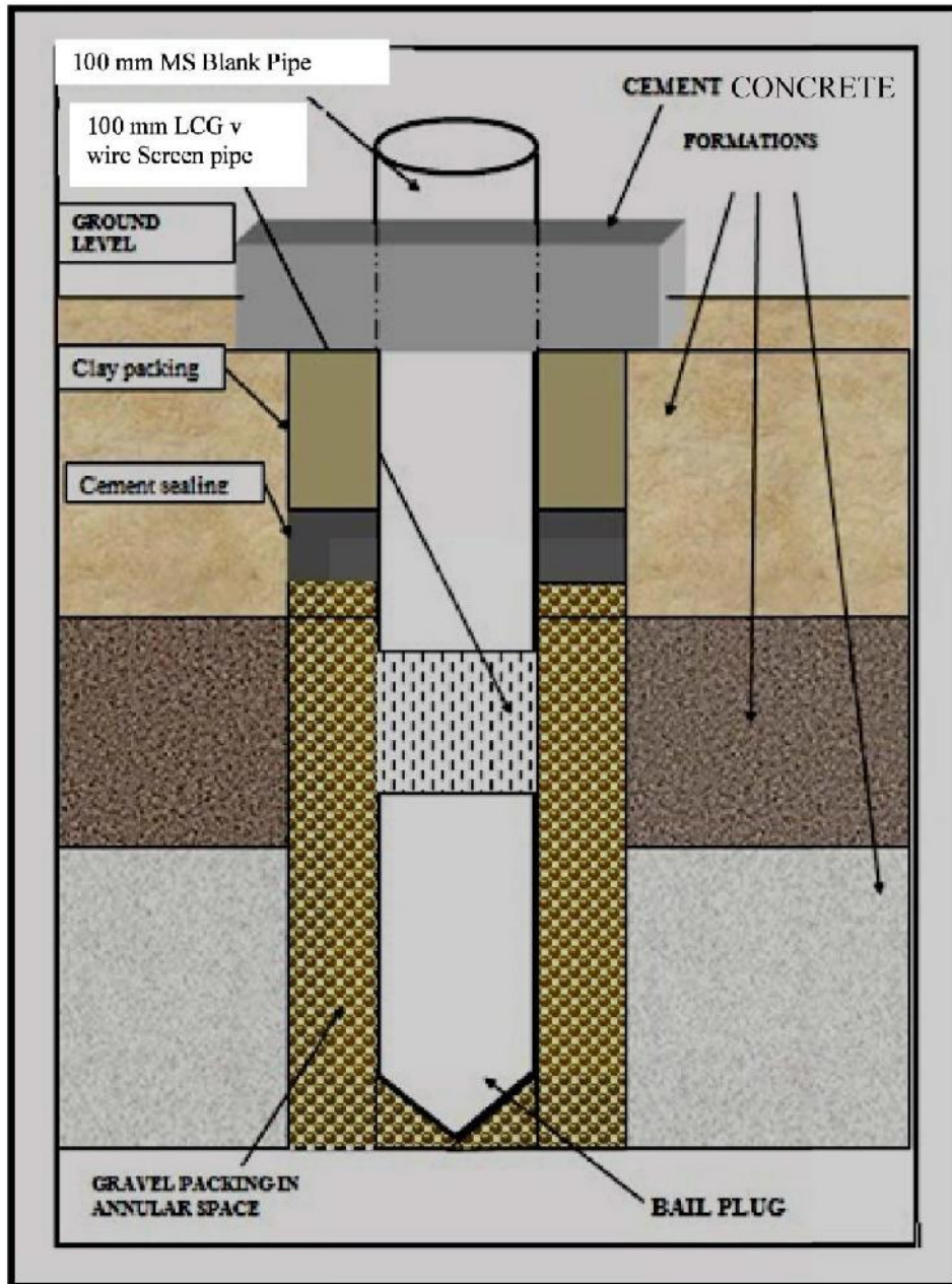
Drawing 1: A Schematic Diagram of Piezometer
