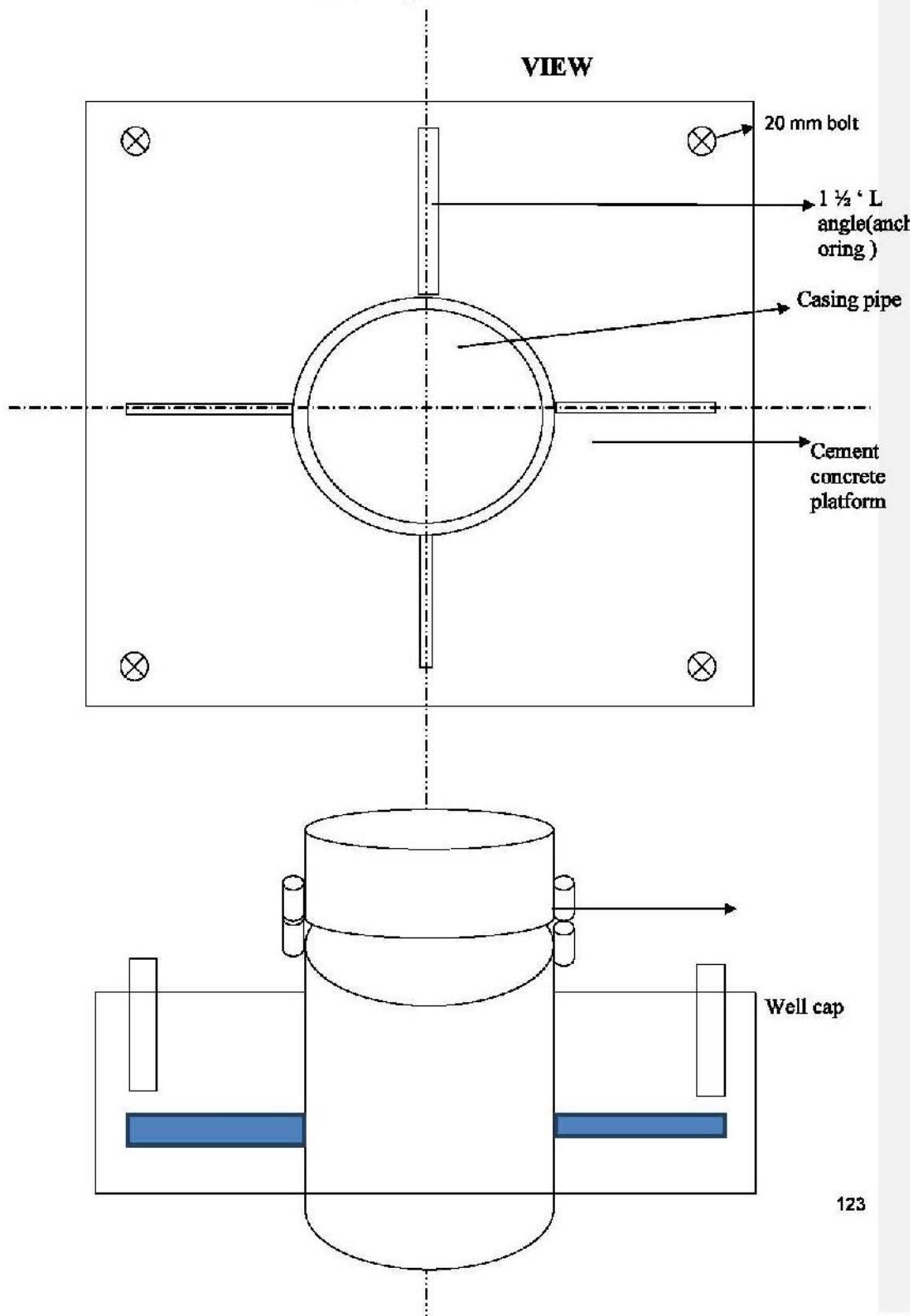
Drawing 4: A Schematic Diagram Cement/Concrete Platform & Well Cap
